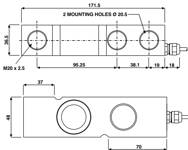
DIMENSIONS FOR CAPACITY 3000kg
